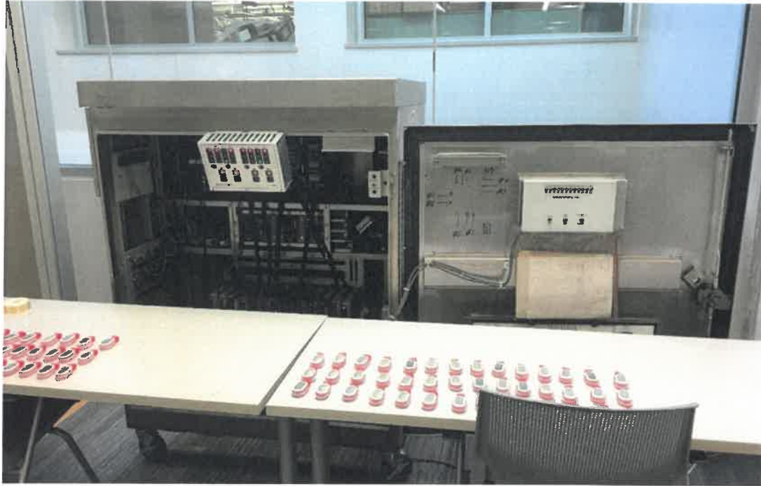
Figure 16: Full-size traffic signal cabinet
